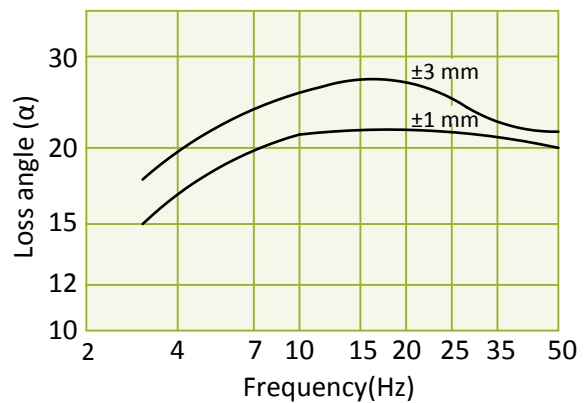
Dynamic damping characteristics of a Hydro mount
